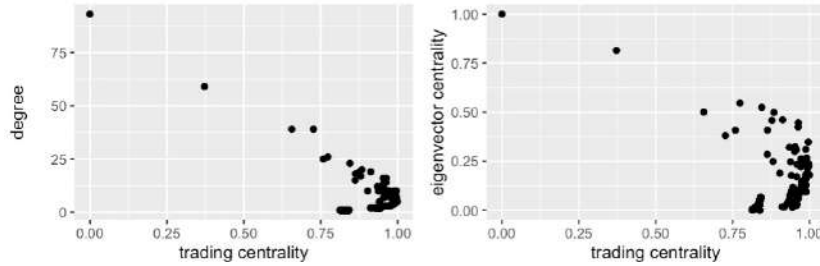
Figure 14: Trading centrality and degree relationship (left); and Trading centrality and eigenvector centrality relationship (right)
