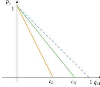
Figure 8: Demand schedules are determined by traders' centrality. The orange demand is of a trader with lower trading centrality; and the green demand is of a trader with higher trading centrality. In blue is the demand schedule if the trading network did not exist.
