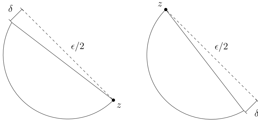
Figure 7: Figure of \epsilon/2 -balls for Lemma 2. As \delta \rightarrow 0 , this sequence approaches the full half circle, which contains a segment of the Pareto frontier.
