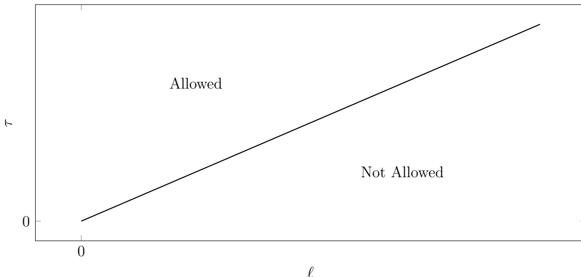
Figure 5: An example of a minimum wage policy. Only contracts above the lines are allowed.
