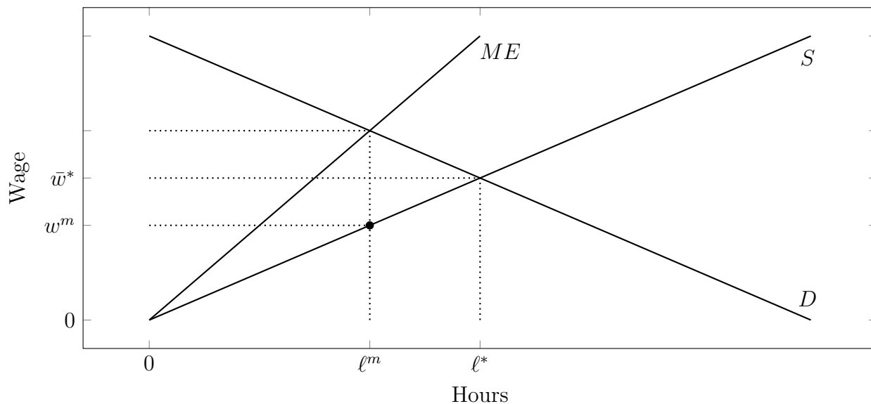
Figure 3: Labor supply, demand, and equilibrium under flexible-hours monopsony. The equilibrium labor hours occur at the intersection between marginal expenditure and labor demand.
