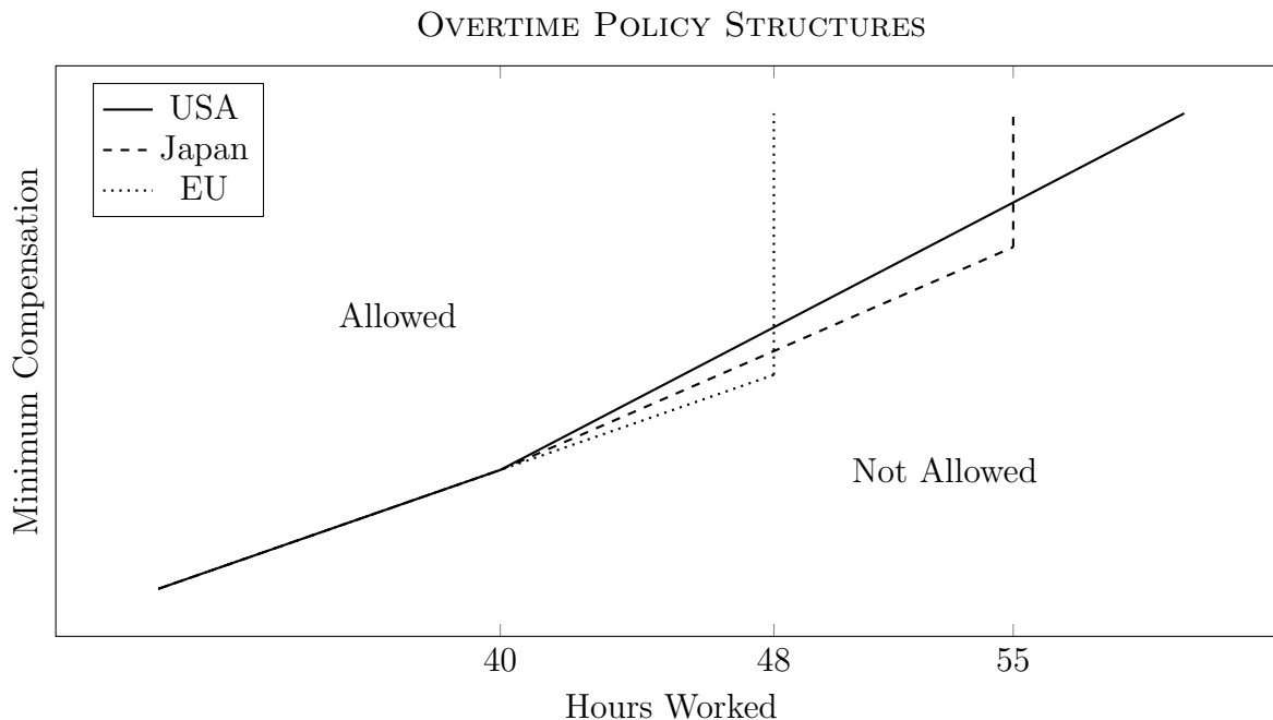
Figure 1: Regulations for minimum total compensation for each number of hours in the United States, Japan, and the European Union with a normalized minimum wage. Contracts with hours and compensation above the line are allowed. Contracts below the line are not.
