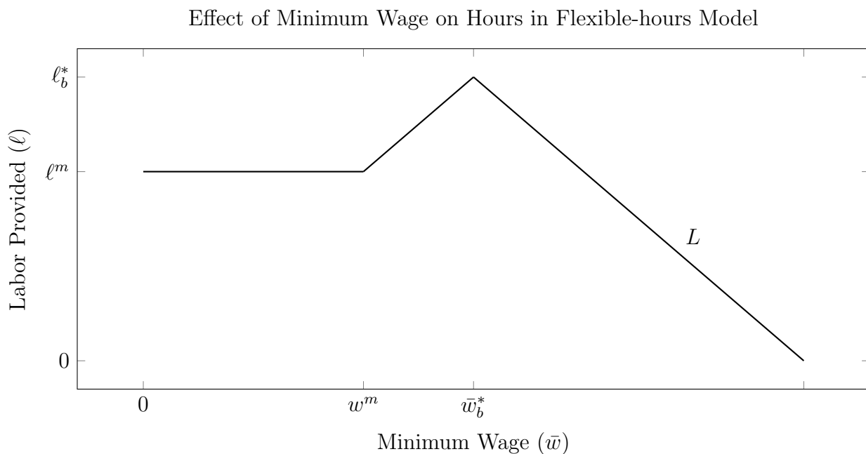
Figure 4: Plot of labor response curve, L for the flexible-hours model. For any minimum wage \bar{w} \in (c'(\ell^m), c'(\ell_b^*)) , the worker is employed for a quantity of hours between the market employment and the efficient level of employment (the inverse of the marginal cost). The minimum wage \bar{w}_b^* = c'(\ell_b^*) = f'(\ell_b^*) implements efficient employment. Labor is decreasing in the minimum wage for wages above \bar{w}_b^* because the firm's limit on work hours is binding.
