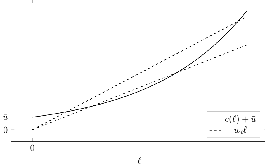
Figure 8: A plot of labor holding the worker's utility constant. The lower intersections are contracts that underemploy the worker while the intersections at the upper part of the curve overemploy the worker at the same wages.
