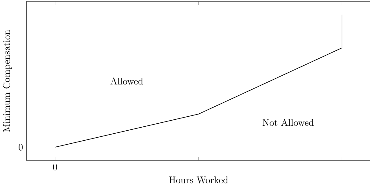
Figure 2: The never Pareto dominated satisficing policy combines a minimum wage, overtime pay, and a cap on hours. This policy guarantees the worker at least as much utility as the contract at the “kink”.
