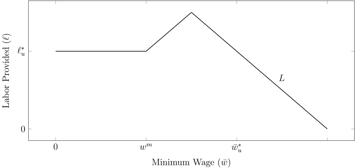
Figure 6: Plot of labor response curve, L for the ultimatum model. It has the same shape as the flexible-hours model in Figure 4. However, for any minimum wage \bar{w} \in (c(\ell_u^*)/\ell_u^*, c'(\ell_u^*)) , the worker is employed for a number of hours that exceeds the efficient quantity. Therefore, the minimum wage that maximizes hours does not implement an efficient allocation.
