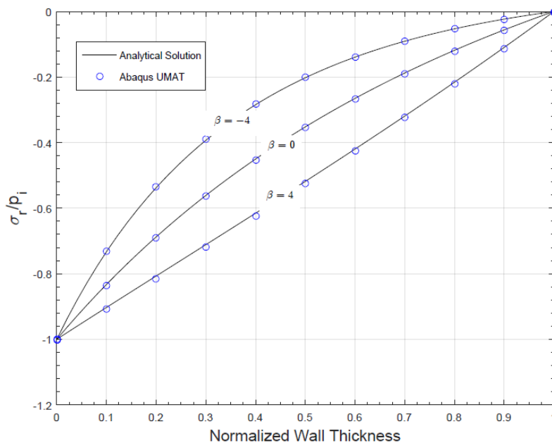
Figure 3 – Radial stress profiles along the pipe wall.
