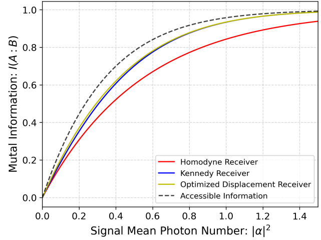
Figure 4: Plot of the mutual information as a function of |\alpha|^2 for the optimized displacement receiver (solid yellow curve), Kennedy receiver (solid blue curve), homodyne receiver (solid red curve). For comparison the accessible information (dashed black curve) is also plotted.
