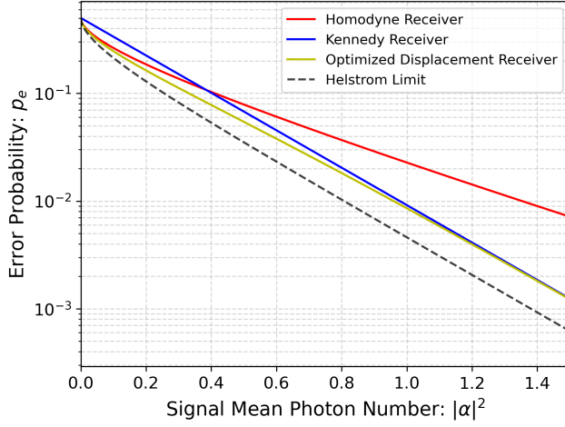
Figure 3: Logarithmic plot of error probability as a function of |\alpha|^2 for the optimized displacement receiver (solid yellow curve), Kennedy receiver (solid blue curve), homodyne receiver (solid red curve), and the Helstrom limit (dashed black curve).
