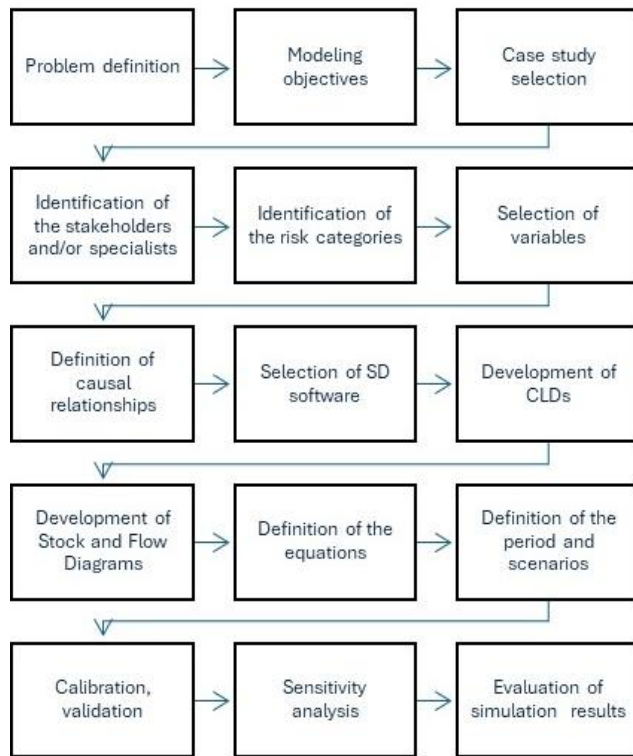
Figure 2. Framework for developing SD modeling for risk management in water utilities.
