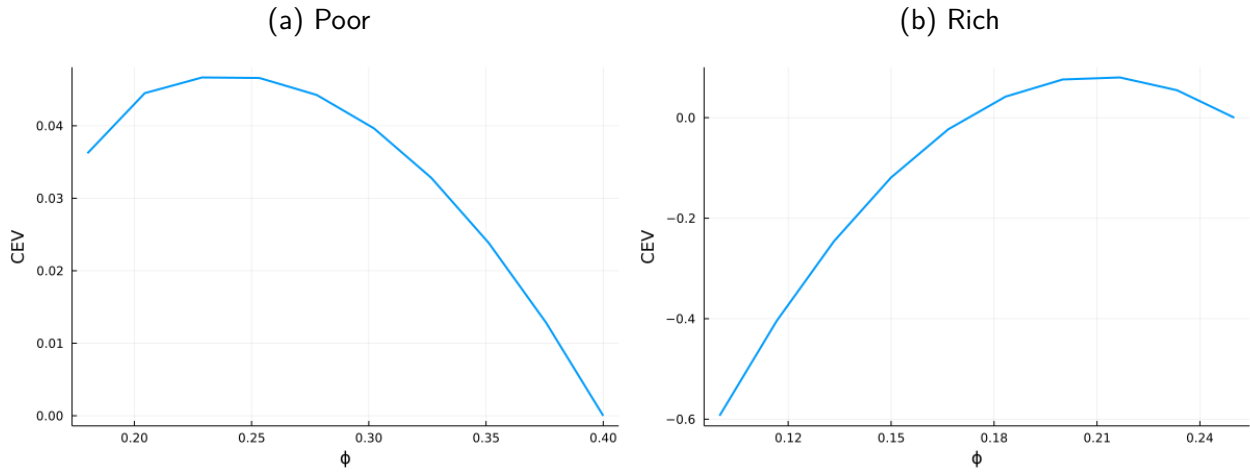
Figure 8: Optimal Progressivity
