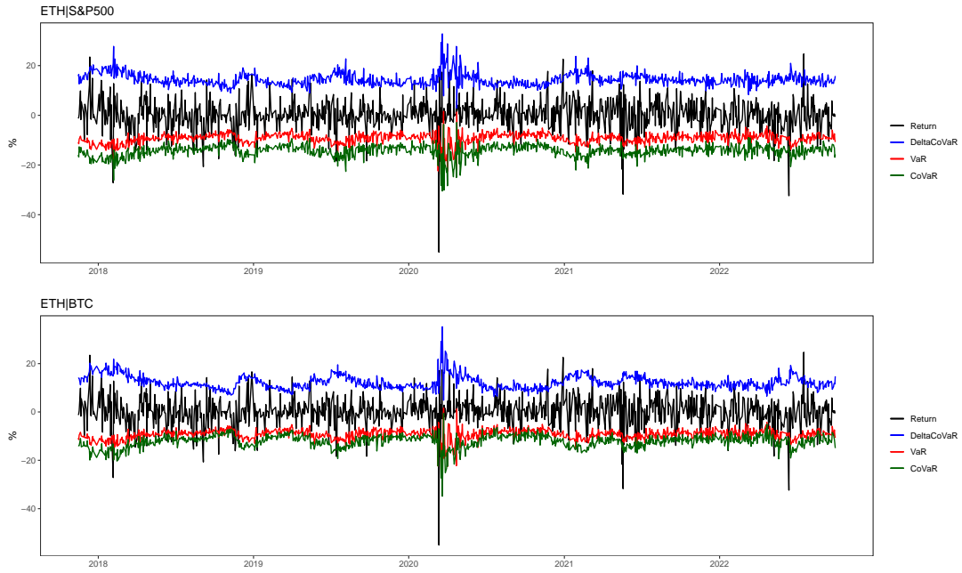
Figure 4. CoVaR and \Delta CoVaR of Ethereum Conditional on S&P500 and Bitcoin
