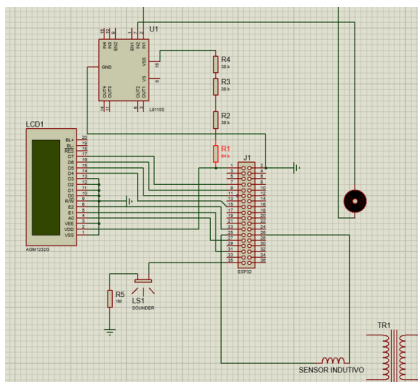
Figure 3. Project schematic showing the sensor actively measuring the metallic object.
