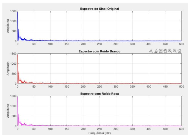
Gráfico 4. Frequency spectrum of signal without and with noise.
