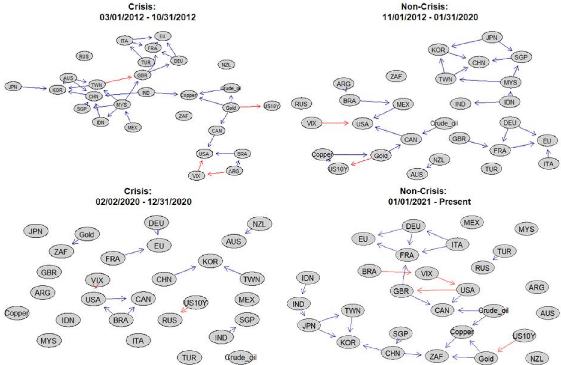
Figure 3 - Dynamic Bayesian Networks (Continued)
