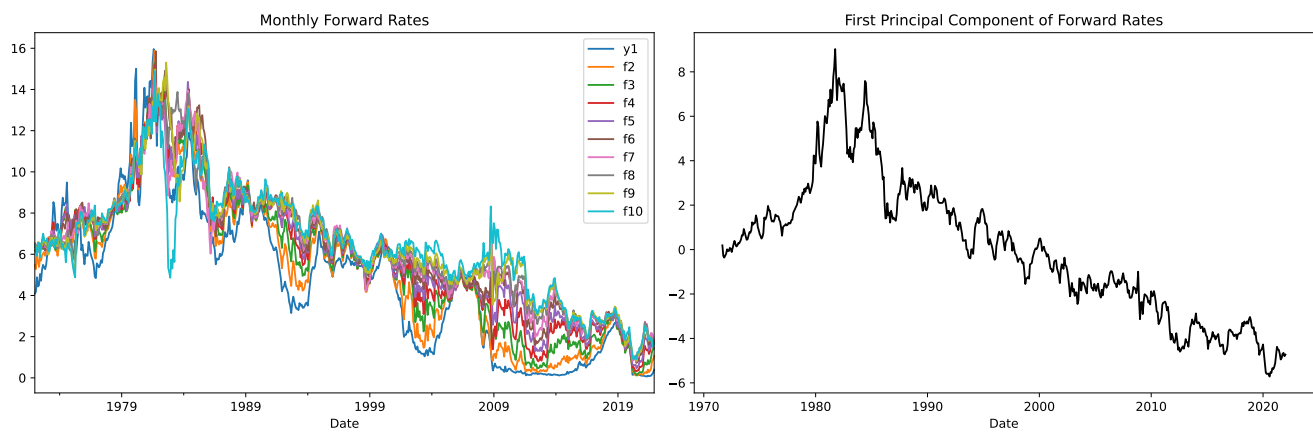
Figure 13: Forward rates and the first principal component. The sample period ranges from January 1973 to December 2021.
