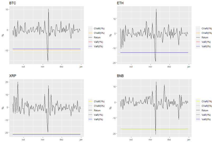
Figure 3 Violations of the returns (Optimal Coupling method).
