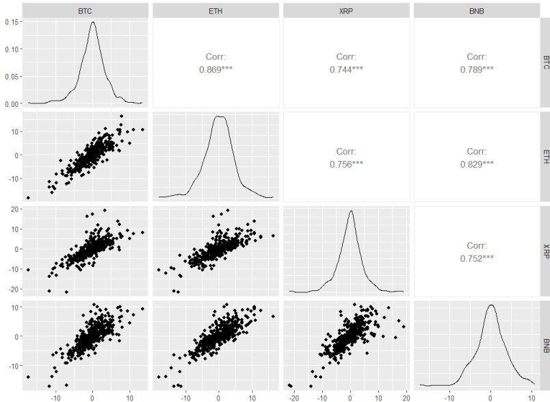
Figure 2 Correlations among the 4-dimensional dataset
