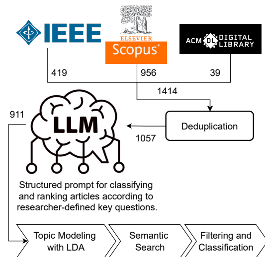
Figure 1: Methodological workflow of the SARA approach. The process begins with corpus deduplication, followed by automatic evaluation of the abstracts through a structured prompt, topic modeling with LDA, and semantic search. In the final stage, articles are filtered, classified, and ranked based on the answers to the researcher’s questions.
