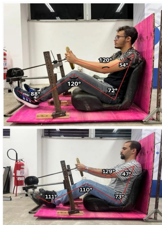
Figure 4: Photogrammetry of the forty-second percentile male (titular drivers) in the ergonomic mockup.
