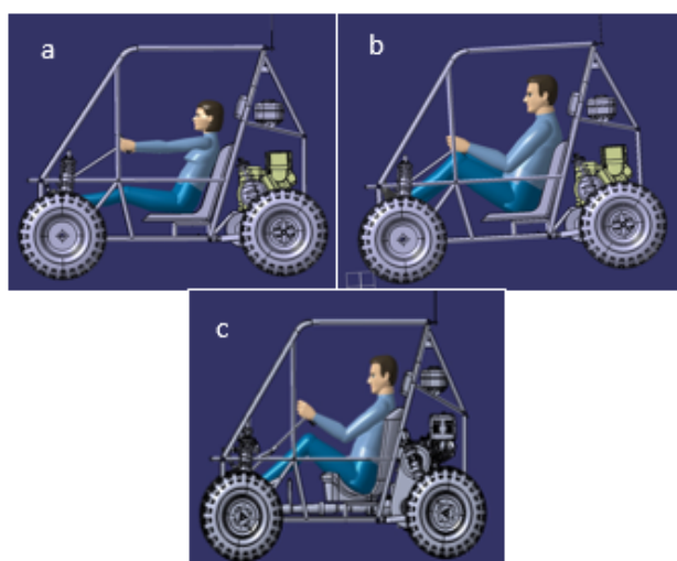
Figure 2: Digital model of ergonomic simulation in CATIA with first (a), ninety-ninth (b), and forty-second (c) percentile drivers.
